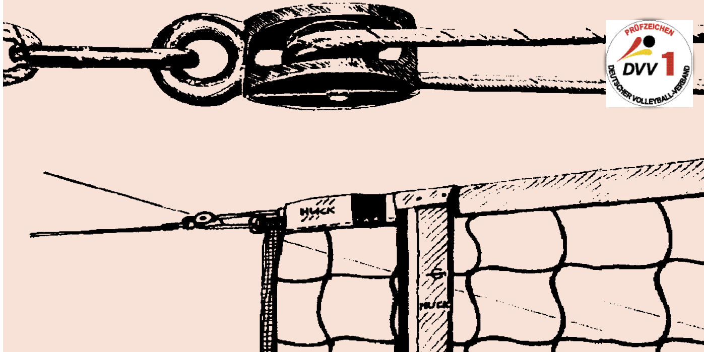
No. 5099: Volleyball Tournament DVV I competition nets. The pulley on each side of the net ensures a perfectly even tension over the entire area of the net.
