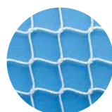
202-020-02 Translucent Knotless Bird Protection Net made from High Tenacity Polypropylene 1mm approx diameter, 20mm mesh
