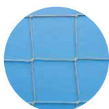
202-050-08 Stone Knotless Bird Protection Net made from High Tenacity Polypropylene 1mm approx diameter, 50mm mesh
